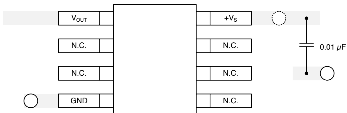
Figure 28. Layout Example
