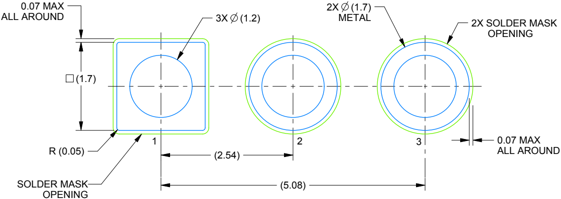
LAND PATTERN EXAMPLE NON-SOLDER MASK DEFINED SCALE:15X
