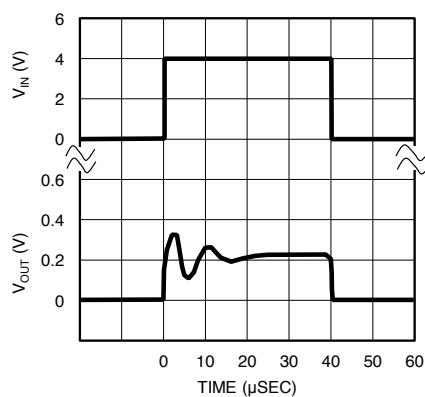
Figure 11. Start-Up Response
