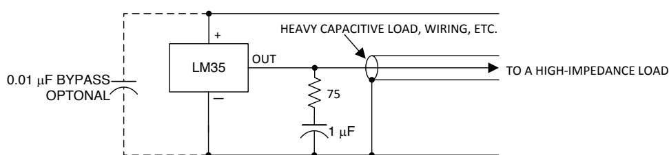
Figure 13. LM35 with R-C Damper
