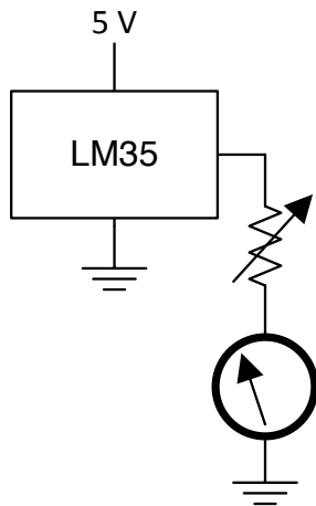
Figure 22. Centigrade Thermometer (Analog Meter)
