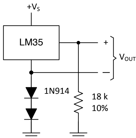
Figure 18. Temperature Sensor, Single Supply ( -55^{\circ} to +150^{\circ}\text{C} )
