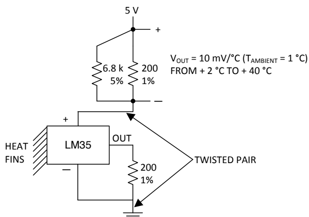
Figure 16. Two-Wire Remote Temperature Sensor (Grounded Sensor)
