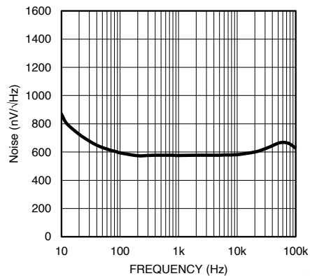
Figure 10. Noise Voltage
