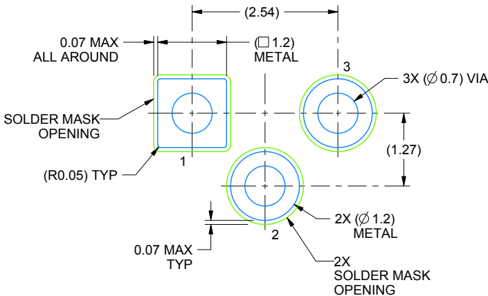
LAND PATTERN EXAMPLE NON-SOLDER MASK DEFINED SCALE:12X
